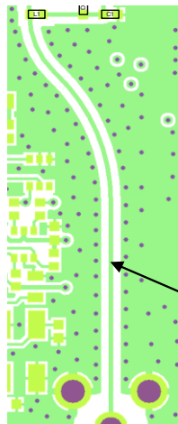
Figure 40: 50\ \Omega grounded coplanar waveguide transmission line designed on the u-blox host PCB bottom layer
