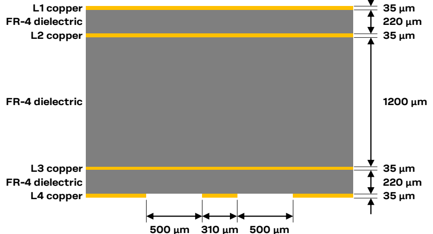
Figure 40: 50\ \Omega grounded coplanar waveguide transmission line designed on the u-blox host PCB bottom layer
