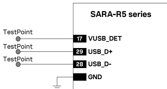
Figure 66: SARA-R5 series modules USB application circuit providing access for diagnostic purpose
