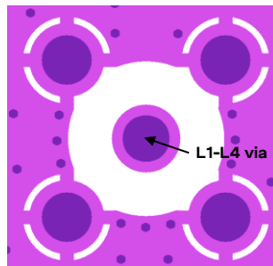
L3 layout
