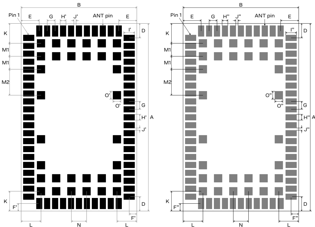
Figure 70: SARA-R5 series modules suggested footprint and paste mask (application board top view)
