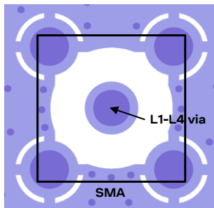
Figure 41: 50\ \Omega SMA female connector layout on the u-blox host PCB
